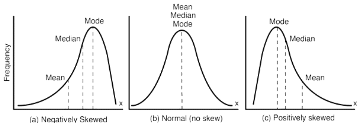
Figure 38: Normal distribution and skewness
