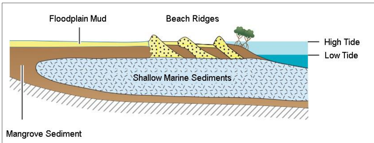
Figure 39: Mangrove sedimentation
