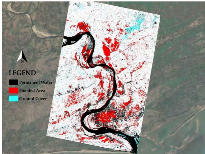
Figure 4 FLOOD HAZARD MAP FOR THE STUDY AREA (SUBARNAREKHA RIVER BASIN, ODISHA, INDIA). DERIVED FLOOD MAP FOR 29 MAY, 2021 FROM SENTINEL-1 SATELLITE IMAGE.
